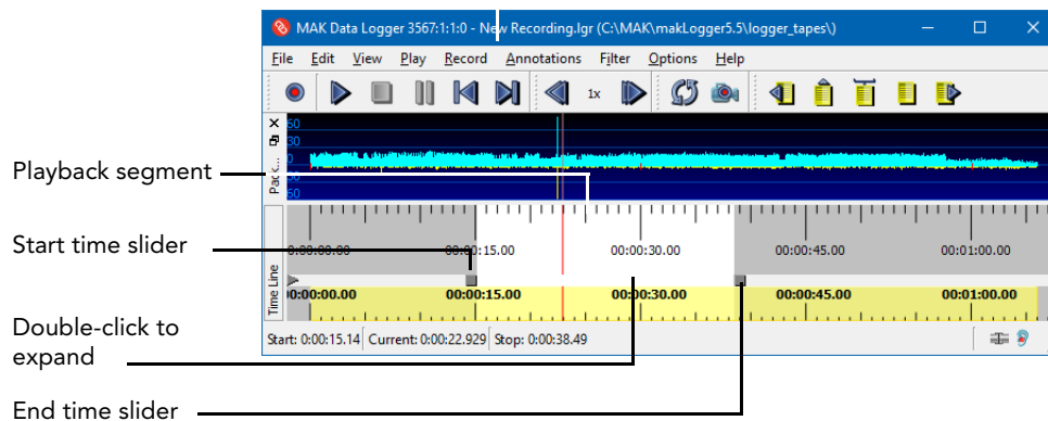
Figure 1-5. Timeline sliders
