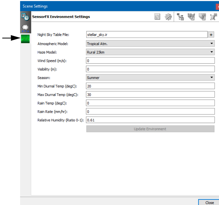
Figure 1-2. SensorFX Environment Settings page
